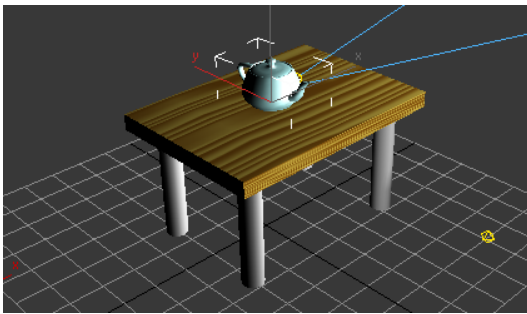
Perspective viewport
