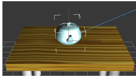
Camera viewport
